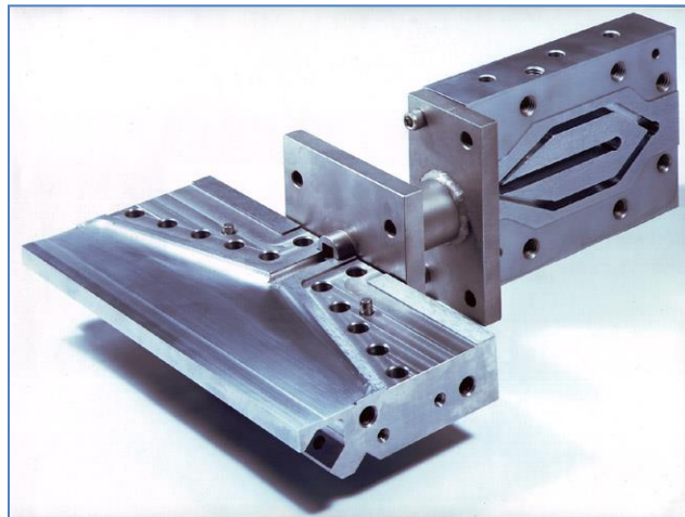
5 Layer coextrusion structure: A-B-A
