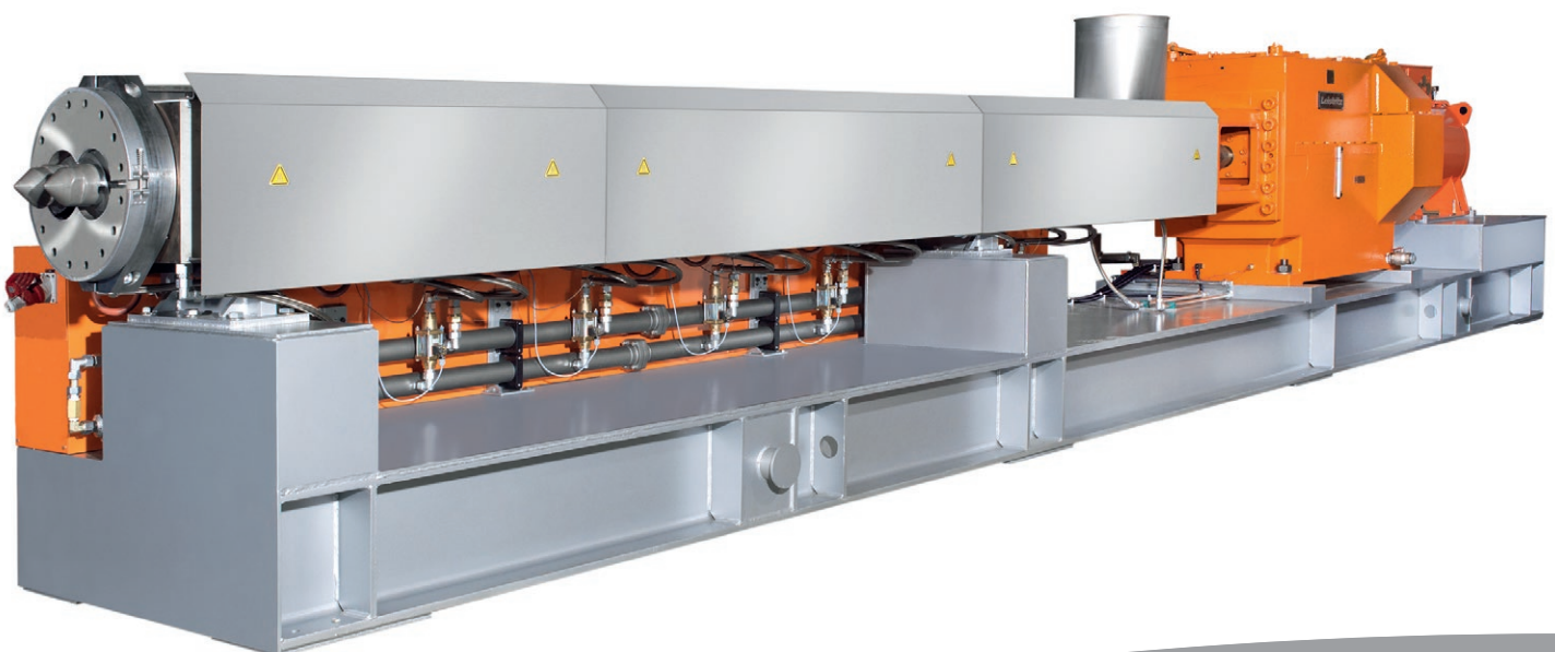
Example of a ZSE 160 MAXX *
