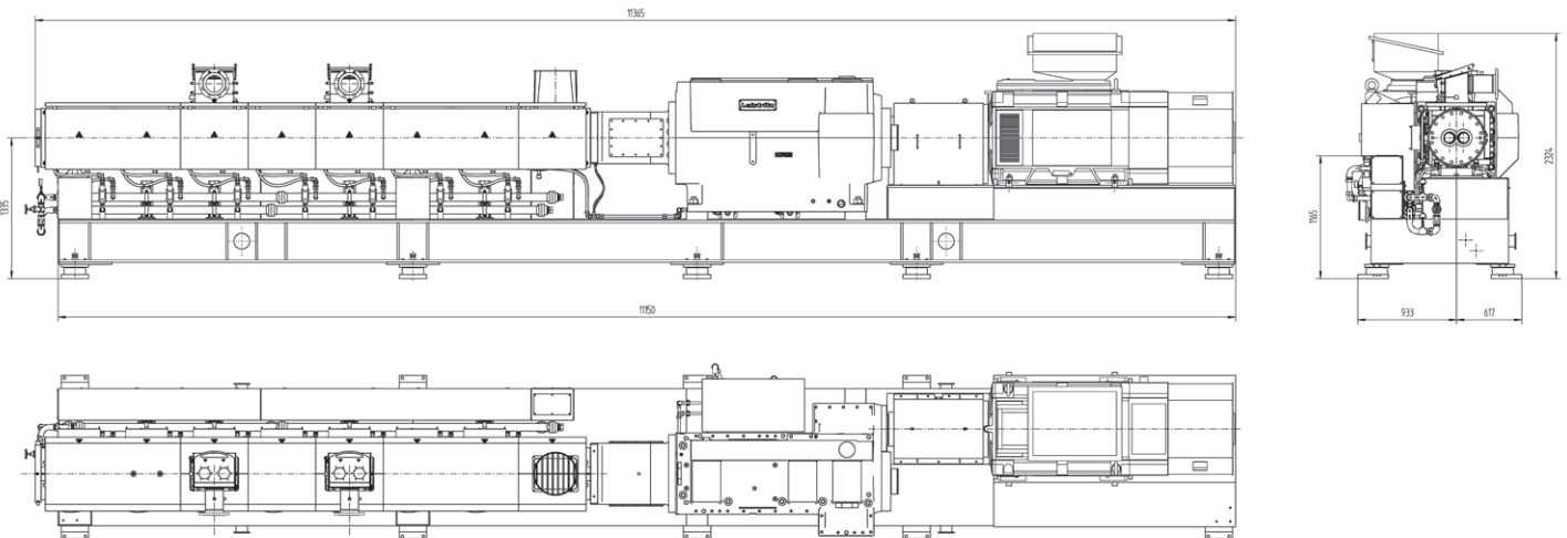
Example of a ZSE 160 MAXX *
